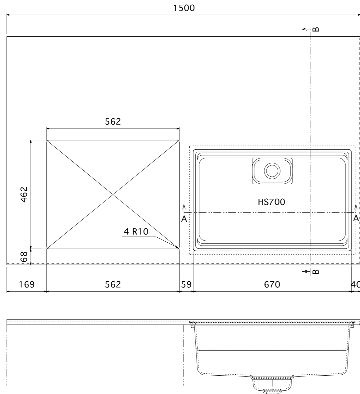
Sec A - A
