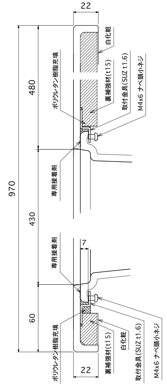
Sec B - B
