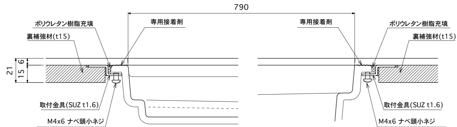
Sec A - A
